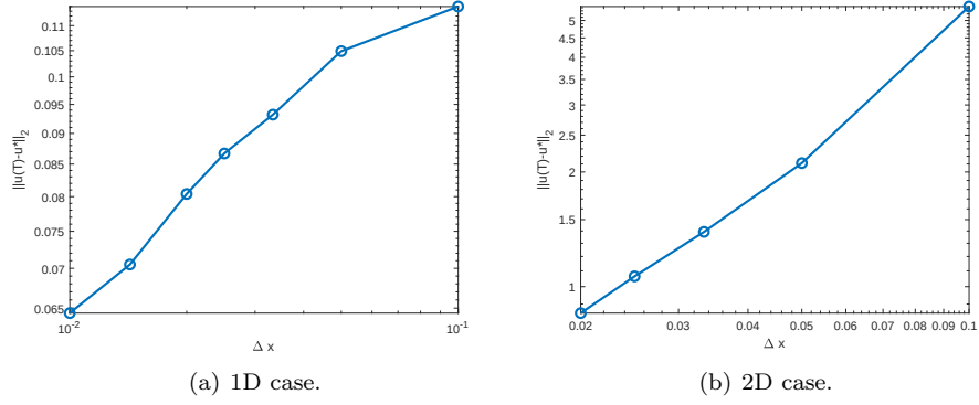
Figure 5: Performance of the gradient descent algorithm 3 as a function of the mesh resolution \Delta x . Left plot corresponds to the one-dimensional case shown in figure 3. There \Delta x = 1/100, 1/70, 1/50, 1/40, 1/30, 1/20, 1/10 , and the total number of iterations is 5000. Right plot corresponds to the two-dimensional case shown in figure 4. There \Delta x = 1/50, 1/40, 1/30, 1/20, 1/10 , and the total number of iterations is 1000.
