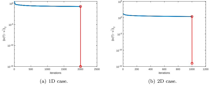
Figure 8: Performance of the adjoint algorithm 4 along iterations. The blue curve shows the evolution of the gradient descent algorithm 3 and the red line shows the improvement made by the least squares postprocessing. Left plot corresponds to the one-dimensional case shown in figure 3. There the computational time is 1.77 seconds and the total number of iterations is 2001. Right plot corresponds to the two-dimensional case shown in figure 7. There the computational time is 115.83 seconds and the total number of iterations is 1001.
